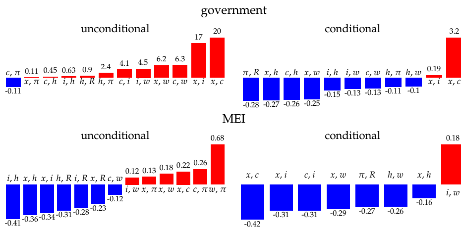
Figure 4: Largest pairwise information complementarities with respect to the government spending and MEI shocks, full spectrum.
