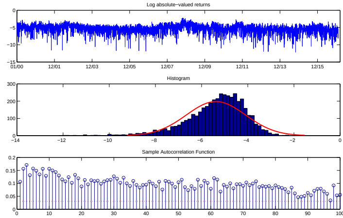
Figure 1: Time-series dynamics, sample histogram (confronted with the theoretical normal distribution), and sample autocorrelation function (with asymptotic 95% confidence bands) of the log absolute-valued returns of the SP500 index.
